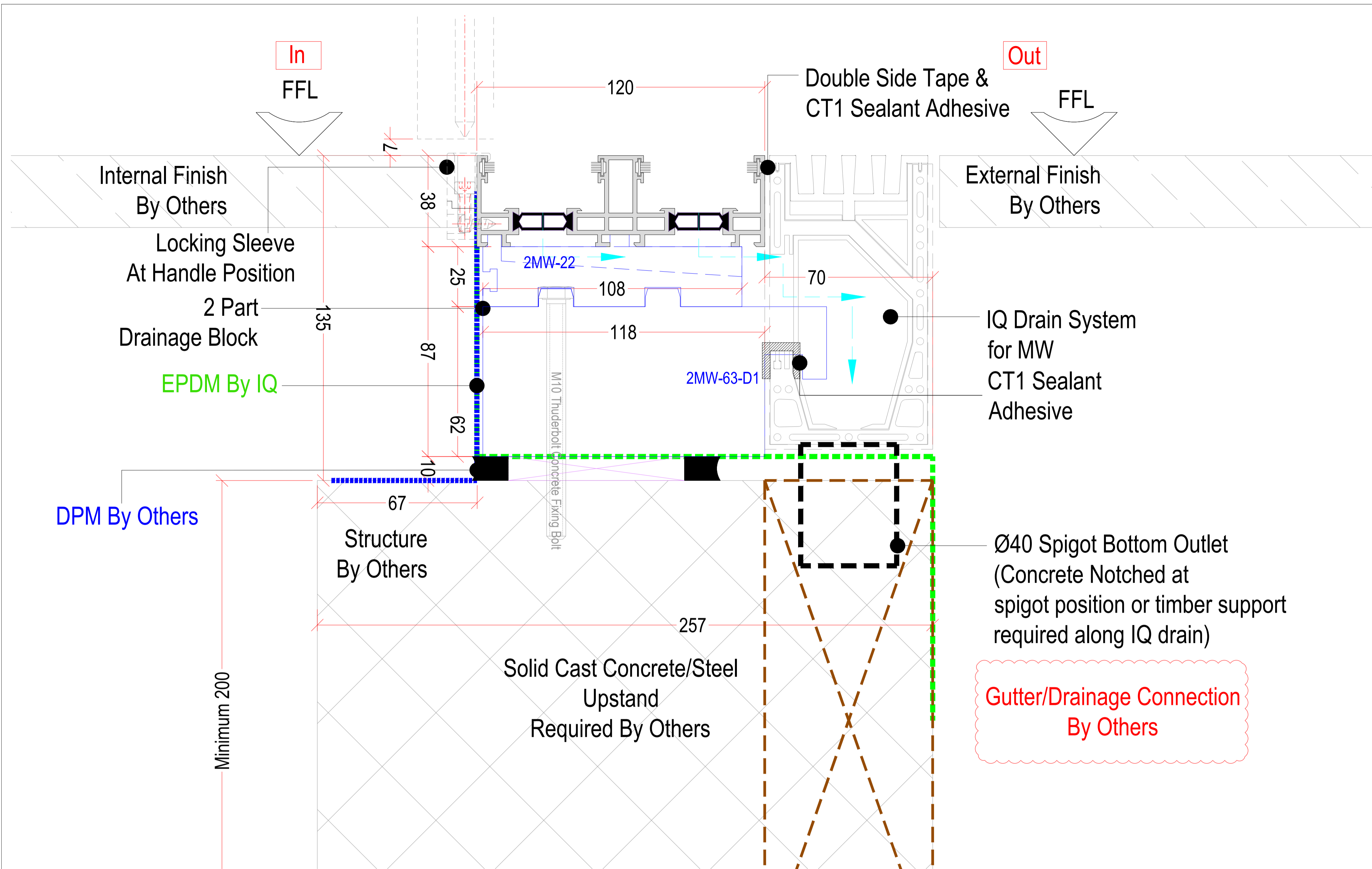
MW - 2 Track Base Detail With IQ Drain Scale 1:1
